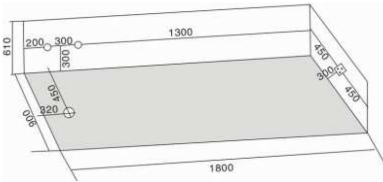
A-3 Bathtub Drawing
